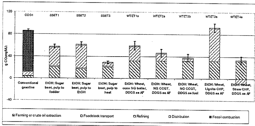
Fig. A1.2: Direct GHG emissions from gasoline and various bioethanol pathways. The main emissions from biofuels are from farming and processing. Unless lignite (brown coal) is used, the GHG balance is positive if no indirect effects are considered.
