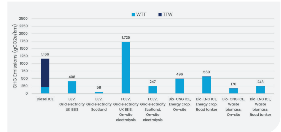
Figure 15. WTW GHG emissions for 18t truck with urban delivery duty cycle ( \text{gCO}_2\text{e/km} ) using different grid electricity GHG emission factors
