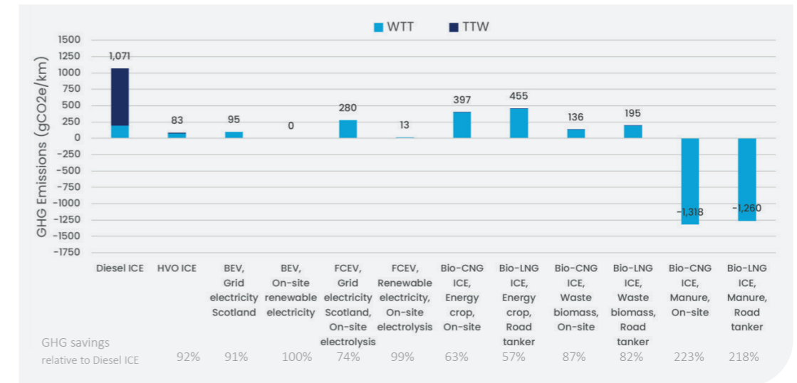
Figure 14. WTW GHG emissions for 44t truck with long haul duty cycle (gCO 2 e/km)
