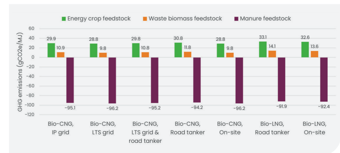
Figure 12. Biomethane WTT GHG emissions (gCO 2 e/MJ)
