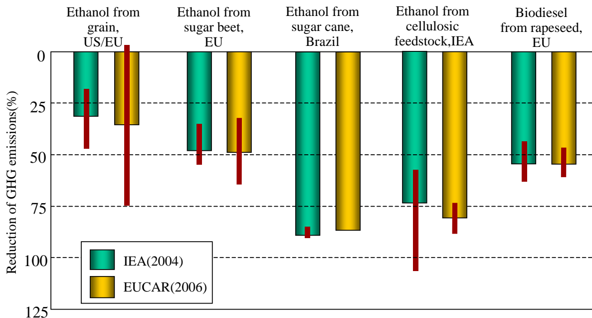
5 Figure 5.10: Reduction of well-to-wheels GHG emissions compared to conventionally fuelled vehicles
