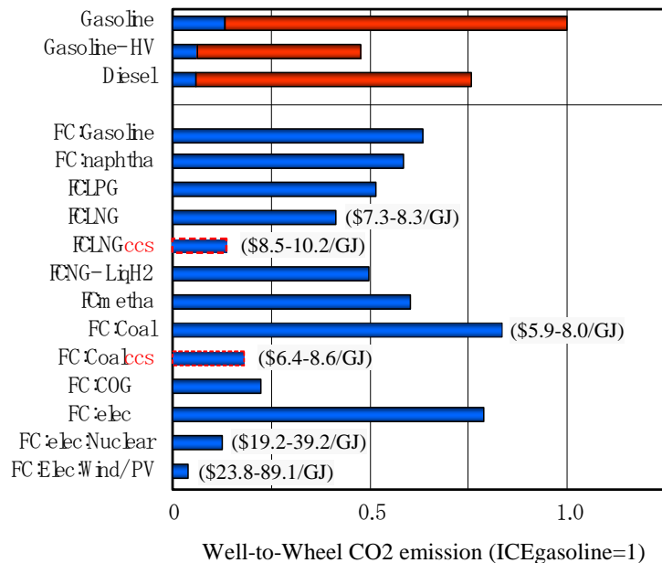
Figure 5.11: Well-to-wheel CO 2 emission for major pathways of hydrogen with some estimates of hydrogen production cost (numbers in parentheses)
