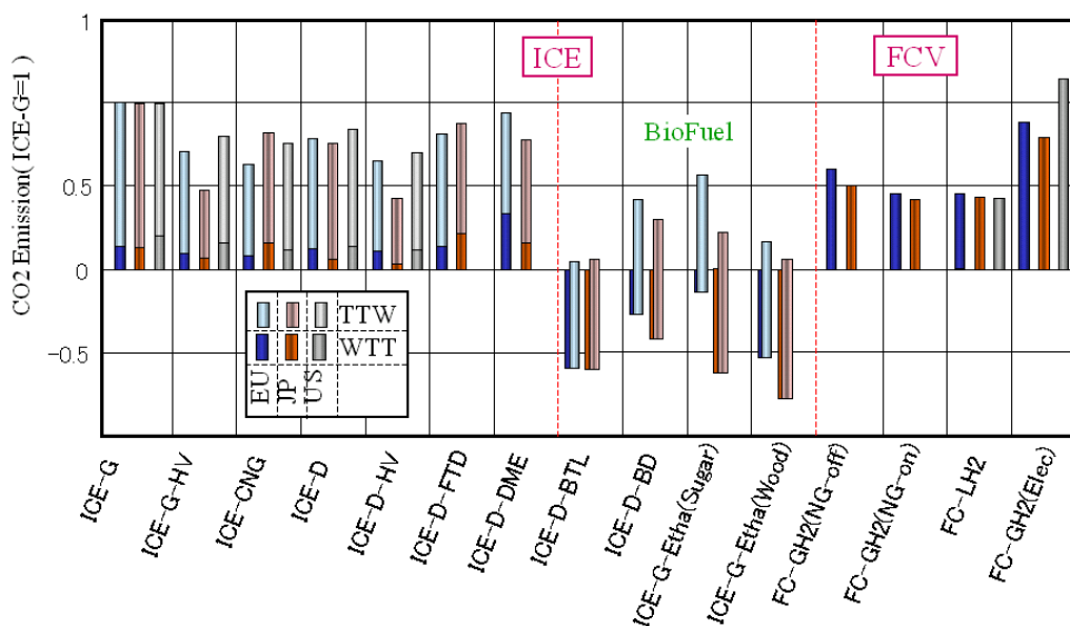
Figure 5.12: Comparison of three studies on Well-to-wheels CO 2 emission analyses Note: See text for an explanation of the legend. All the results are normalized by the value of ICE-G (gasoline). Source: EUCAR/CONCAWE/JRC, 2006; GM/ANL, 2005; Toyota/Mizuho, 2004.
