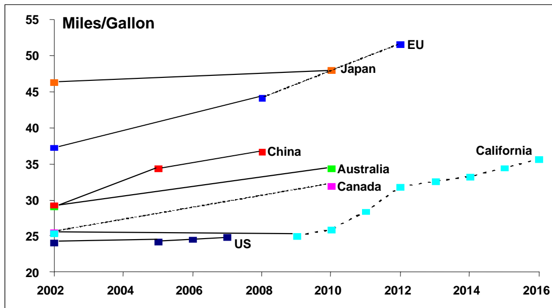
Figure 5.18: Fuel economy and GHG emission standards
