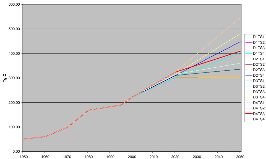
20 Figure 5.7: Historical and projected CO 2 emissions of seagoing shipping, 1990 to 2050 (TgC/yr)
