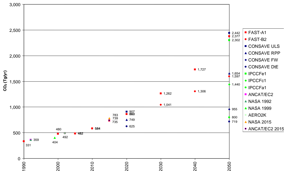
Figure 5.6: Comparison of global CO 2 emissions of civil aviation, 1990–2050
