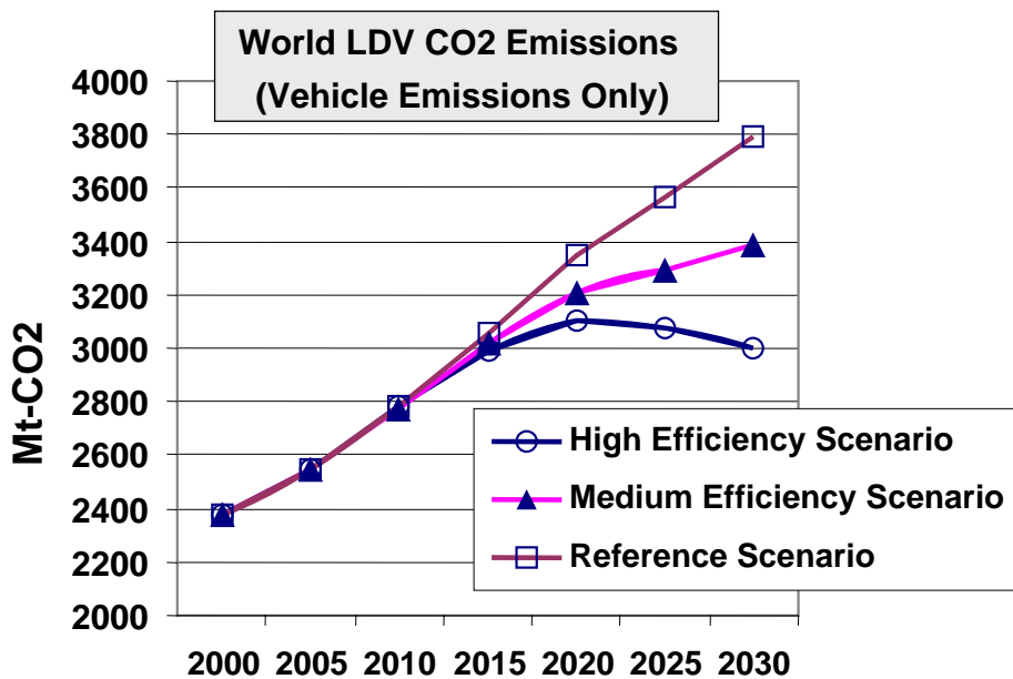
Figure 5.16: Light-duty vehicle CO 2 emissions for three scenarios
